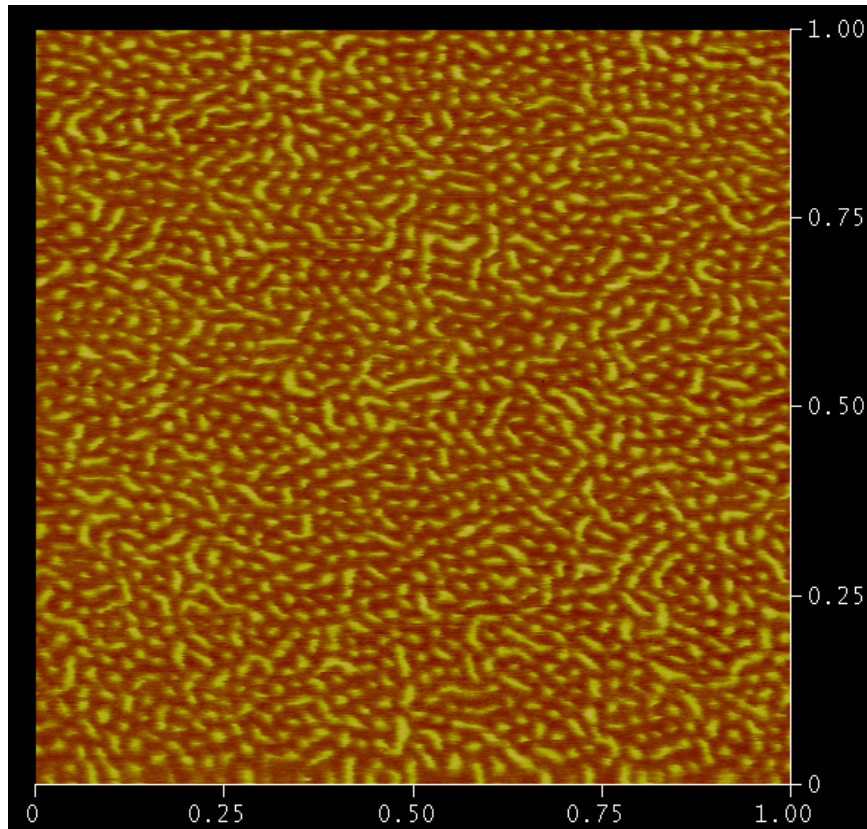
IS-diblock copolymer (IS-06, wt% 79/21), scale: \mu\text{m}
