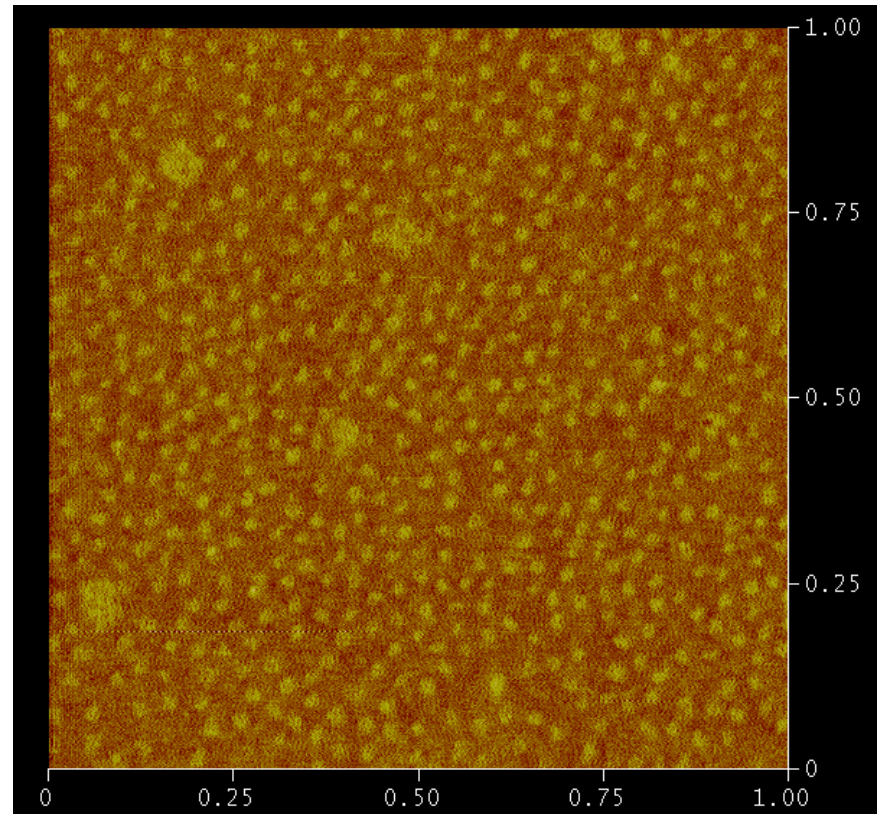
Fluorinated IS diblock copolymer (FIS-06, wt% 86/14), scale: \mu\text{m}
